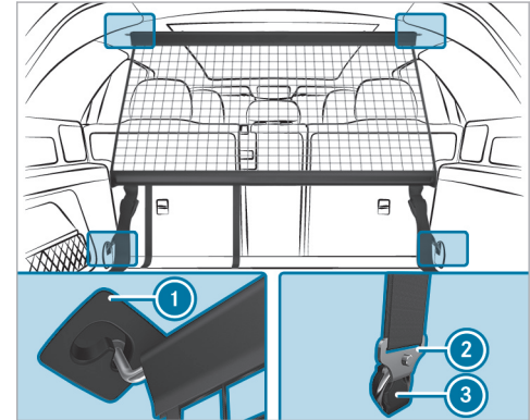
Partitioning net without cargo compartment enlargement
