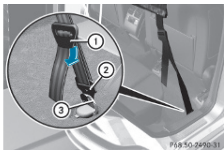
Belt hook attached behind the front seats
