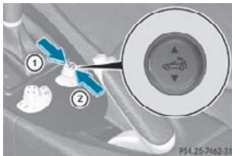
Retractable hardtop switch
