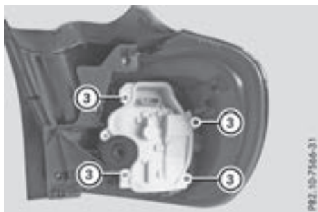
Tail lamps
