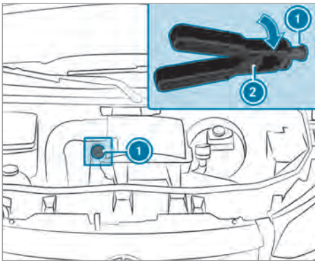
Example: jump-start connection
