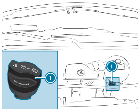
OM654 engine
