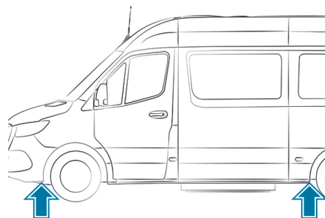
Jack support points
