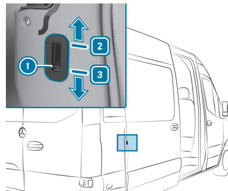
Example: sliding door child safety lock
