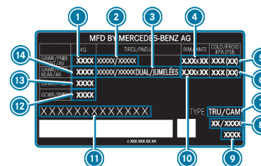
Vehicle identification plate (example: Canada, complete vehicles)
